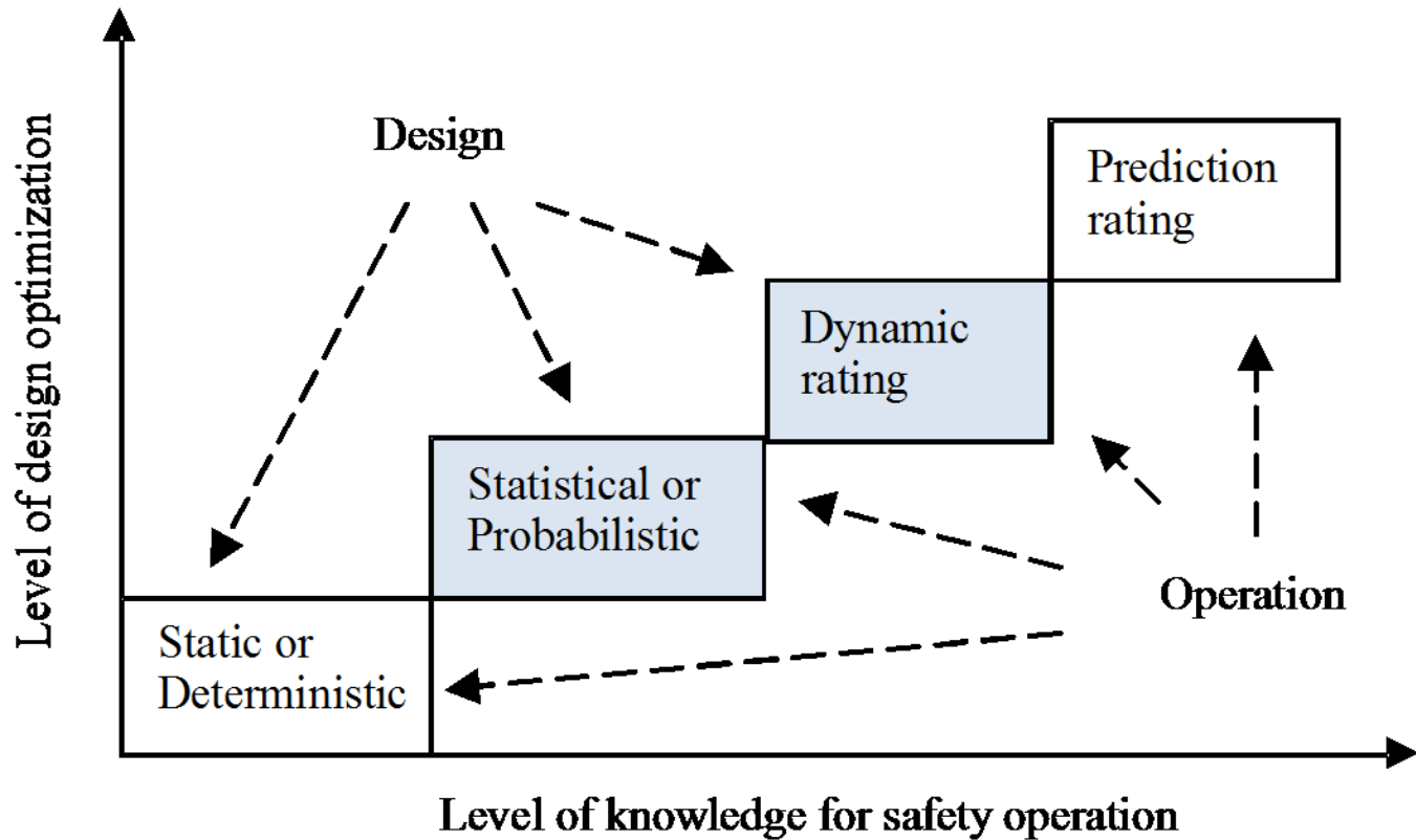
i) Pattern of ampacity model criteria
